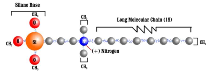
Organo Silane
